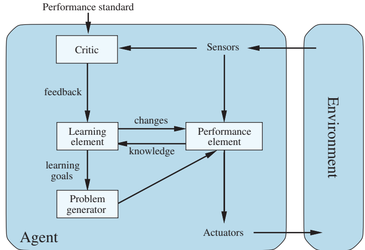
Figure 2.15 A general learning agent. The “performance element” box represents what we have previously considered to be the whole agent program. Now, the “learning element” box gets to modify that program to improve its performance.
